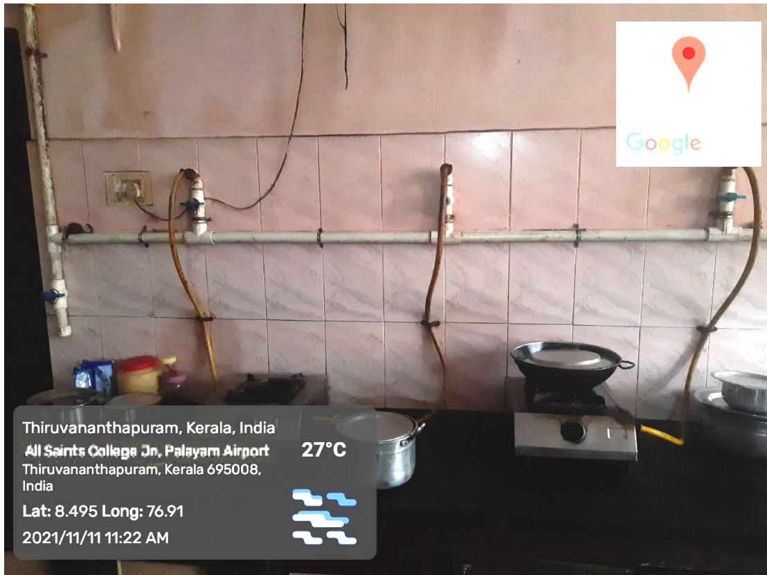
RETICULATED BIOGAS SUPPLY AT THE ALL SAINTS' COLLEGE HOSTEL
